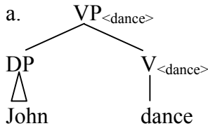
(15) Unergative
