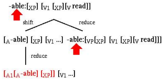
Figure 7: Read-able SHIFT/REDUCE conflict
