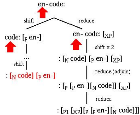
Figure 8: En-code SHIFT/REDUCE conflict
