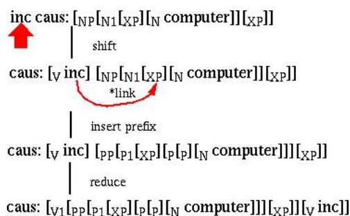
Figure 10: Example of empty prefix insertion
